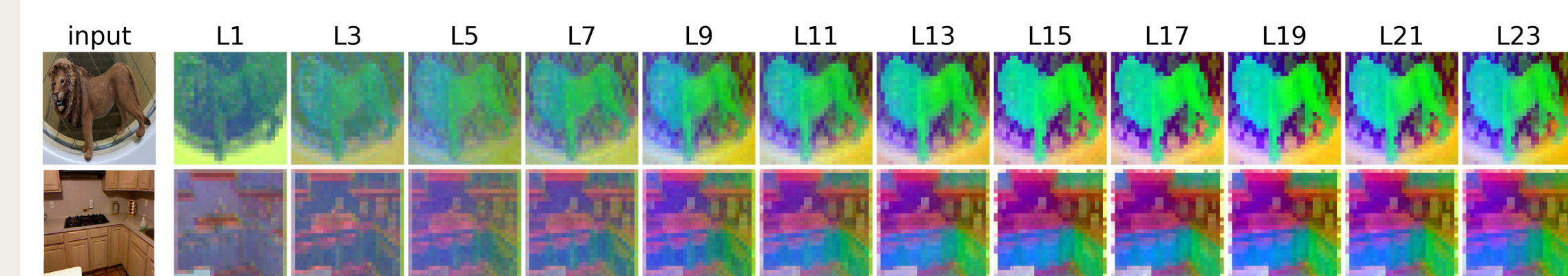
Fig. 3: MAE-L (one PCA per image): with depth, the lion and the kitchen regions become increasingly distinct.
