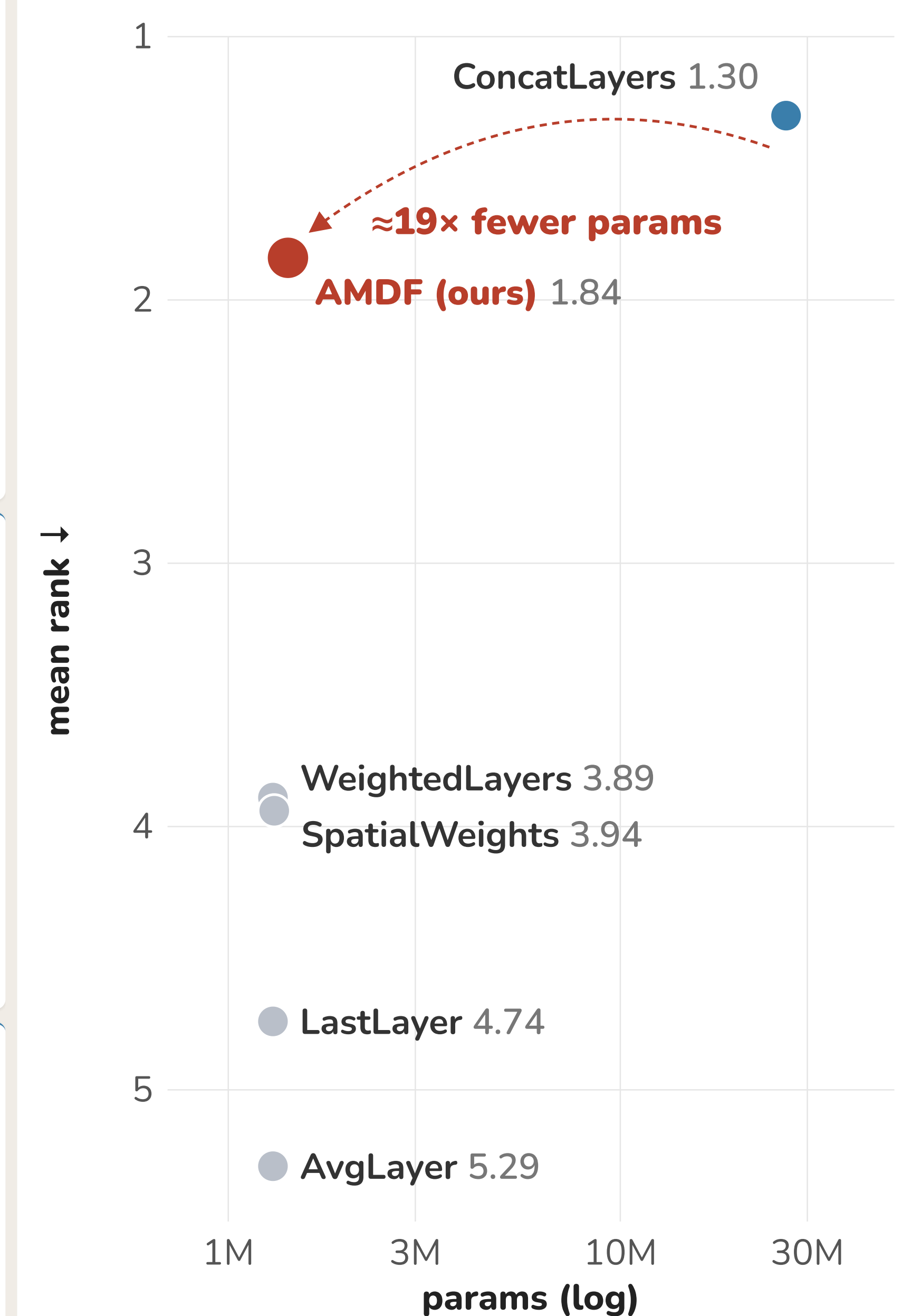
Fig. 7: ViT-L, all 5 tasks: ≈19x (pose head larger; ≈22x on dense tasks).
