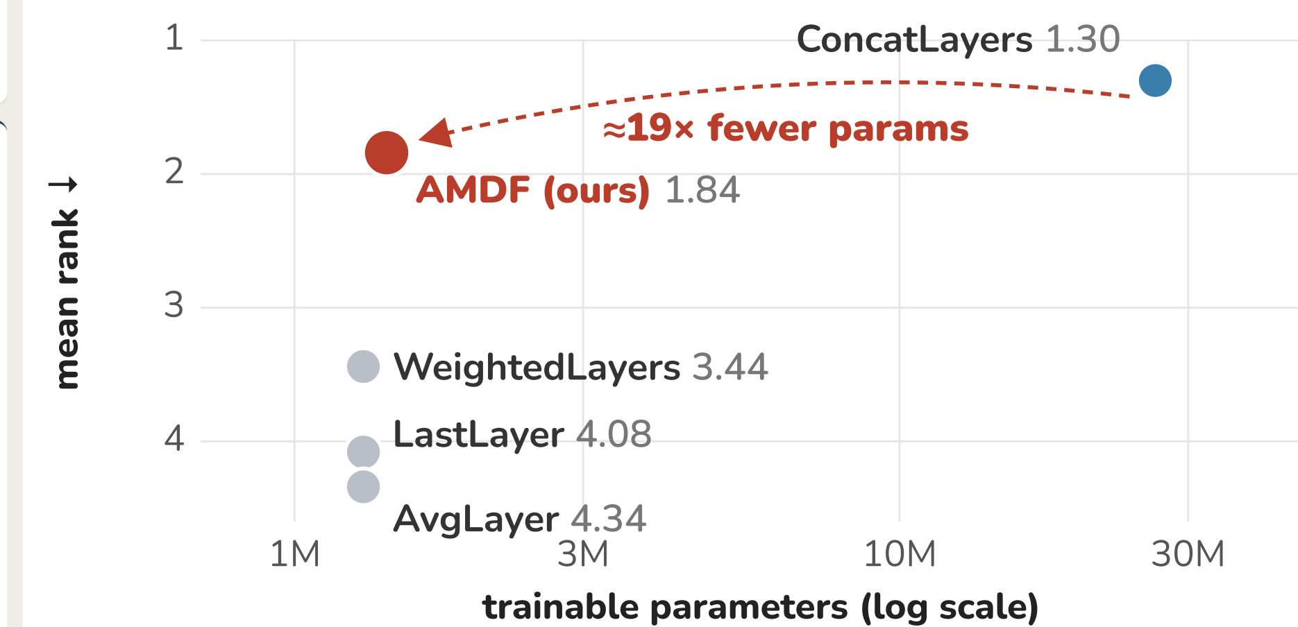
Fig. 6: Mean of the 5 per-table ranks vs. trainable parameters (probe + head, DINOv3-L, averaged over the same tasks; the pose head makes the ratio \approx 19\times here vs \approx 22\times on dense tasks alone).
