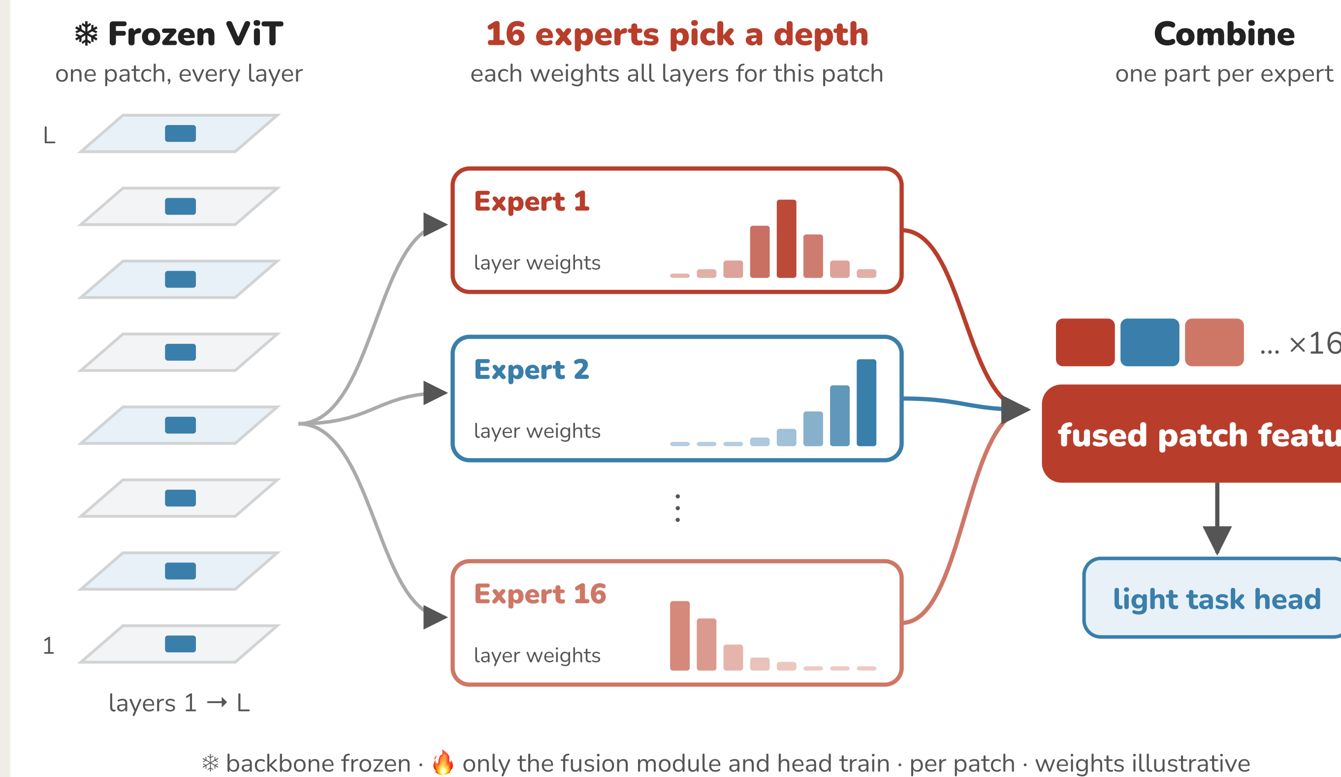
Fig. 1: Geometry peaks mid-depth, semantics at the end; AMDF fuses all layers per patch.
