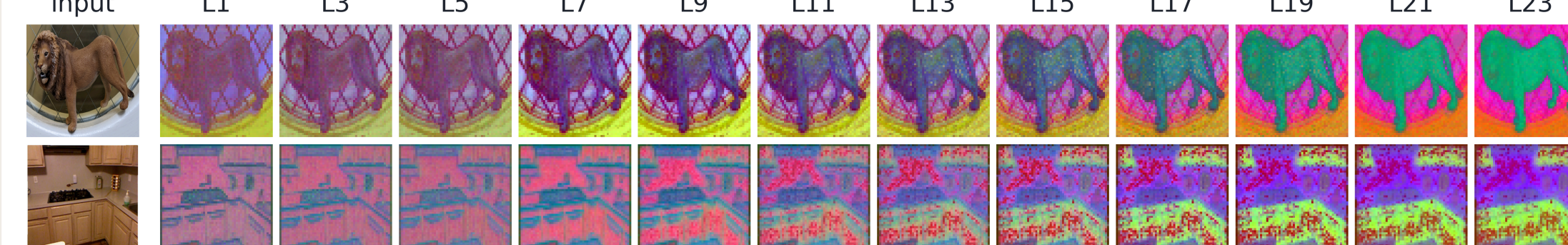
Fig. 3: Layers see differently: frozen PESpatial-L patch features (one PCA per image, 770 px input); object-background separation appears only in deep layers.
