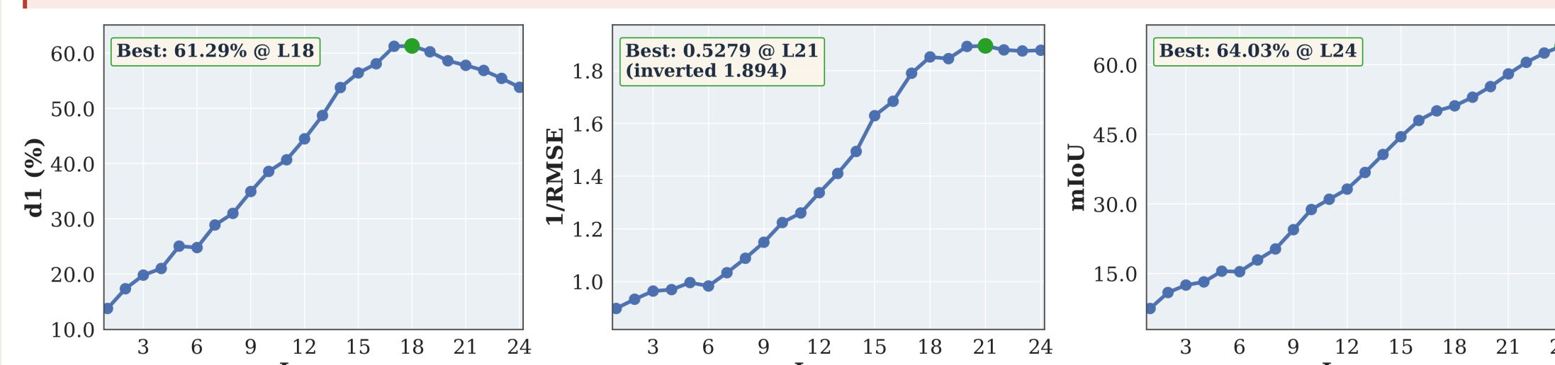
Fig. 2: One probe per layer of a frozen DINOv3-L on NYUv2: the best layer moves deeper as the task gets more semantic (L18 → L21 → L24).
