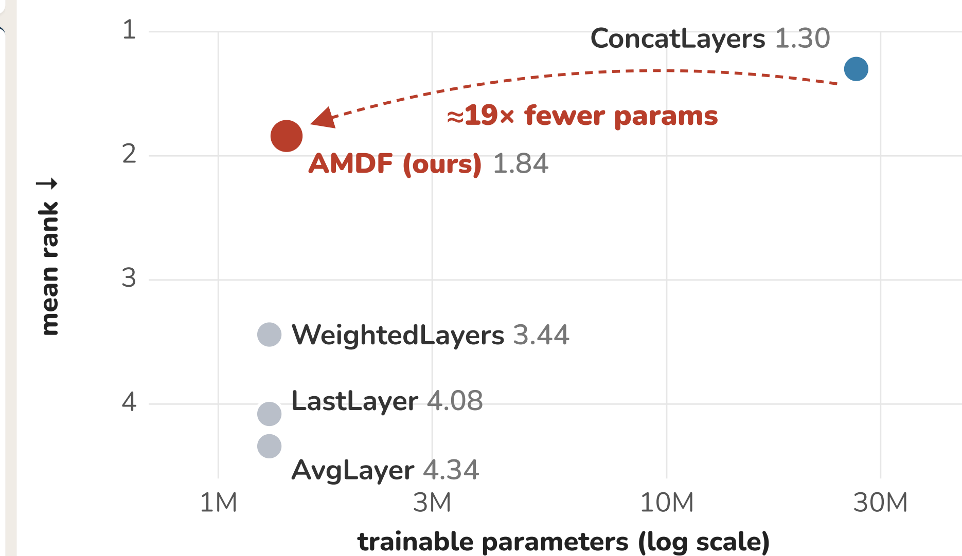
Fig. 6: Mean of the 5 per-table ranks vs. trainable parameters (probe + head, DINOv3-L, averaged over the same tasks; the pose head makes the ratio \approx 19\times here vs \approx 22\times on dense tasks alone).
