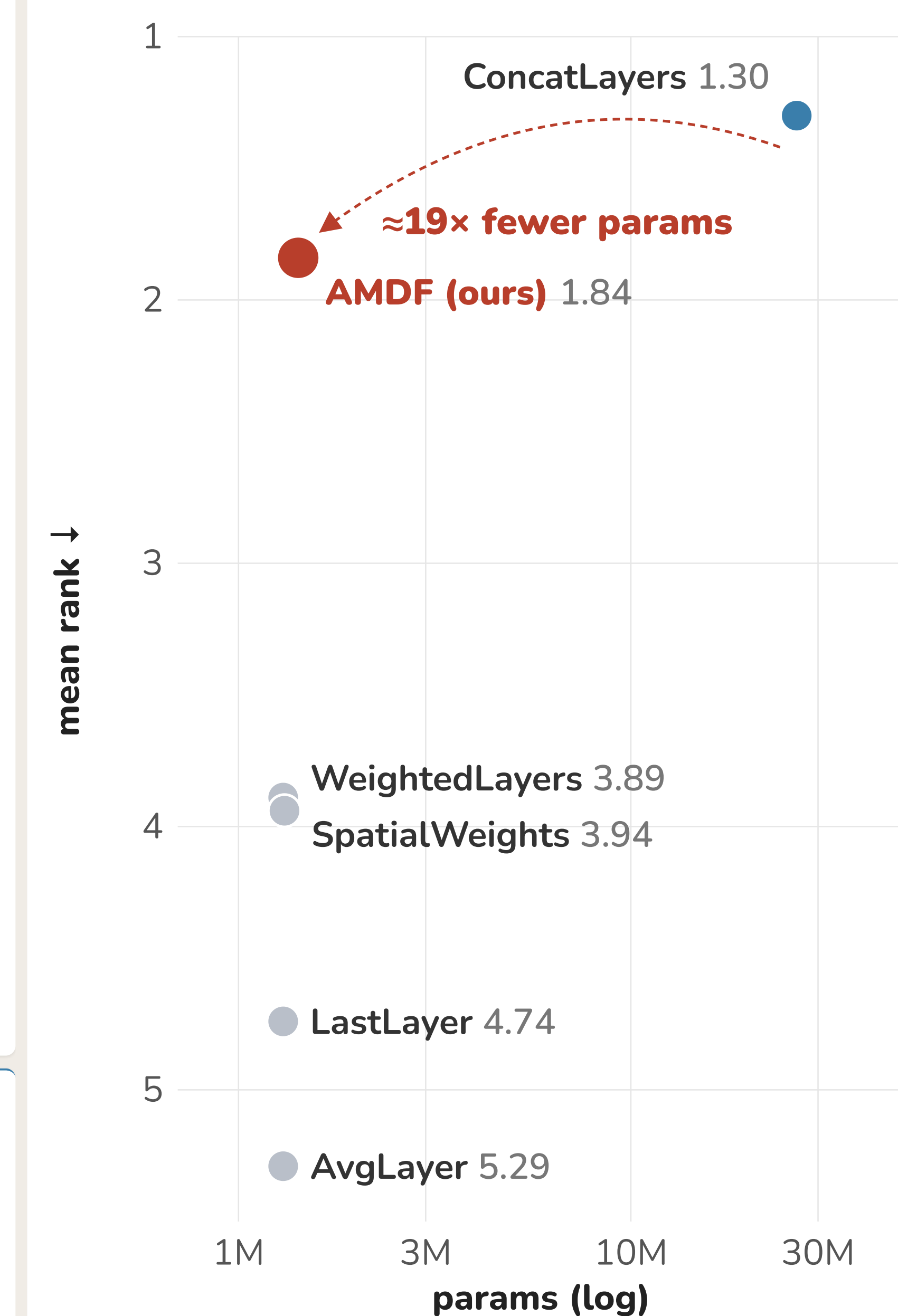
Fig. 6: \approx 19\times fewer params than Concat (5-task average, DINOv3-L).
