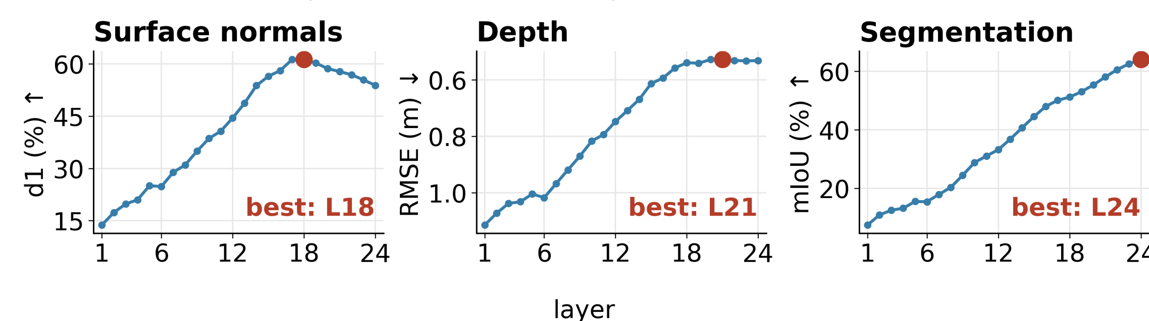
Fig. 2: Best single layer differs per task: \approx L18 (normals), \approx L21 (depth), L24 (segmentation); one seed per layer (DINOv3-L, NYUv2).
