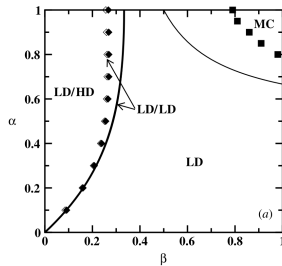
Ours vs original (Pronina & Kolomeisky 2007, Fig. 2)
