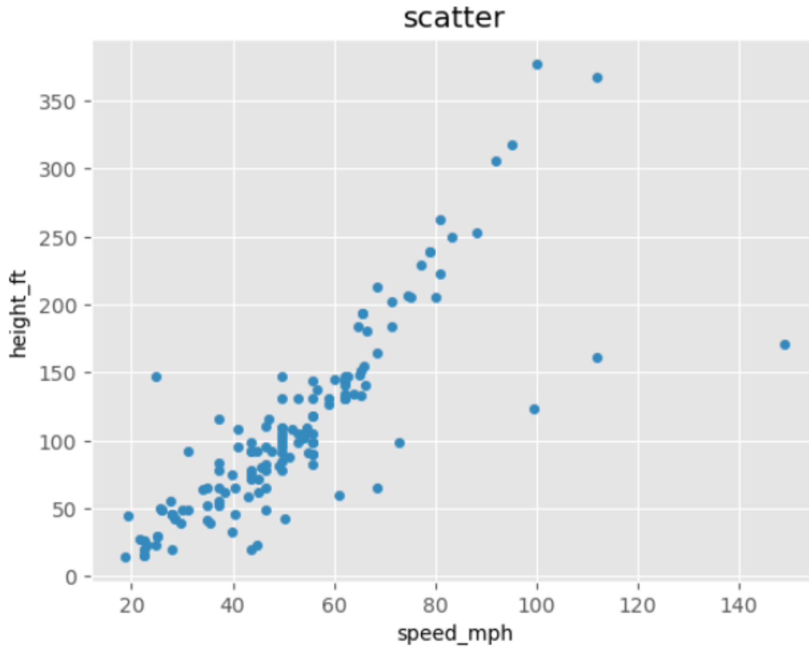
Scatter Plot
