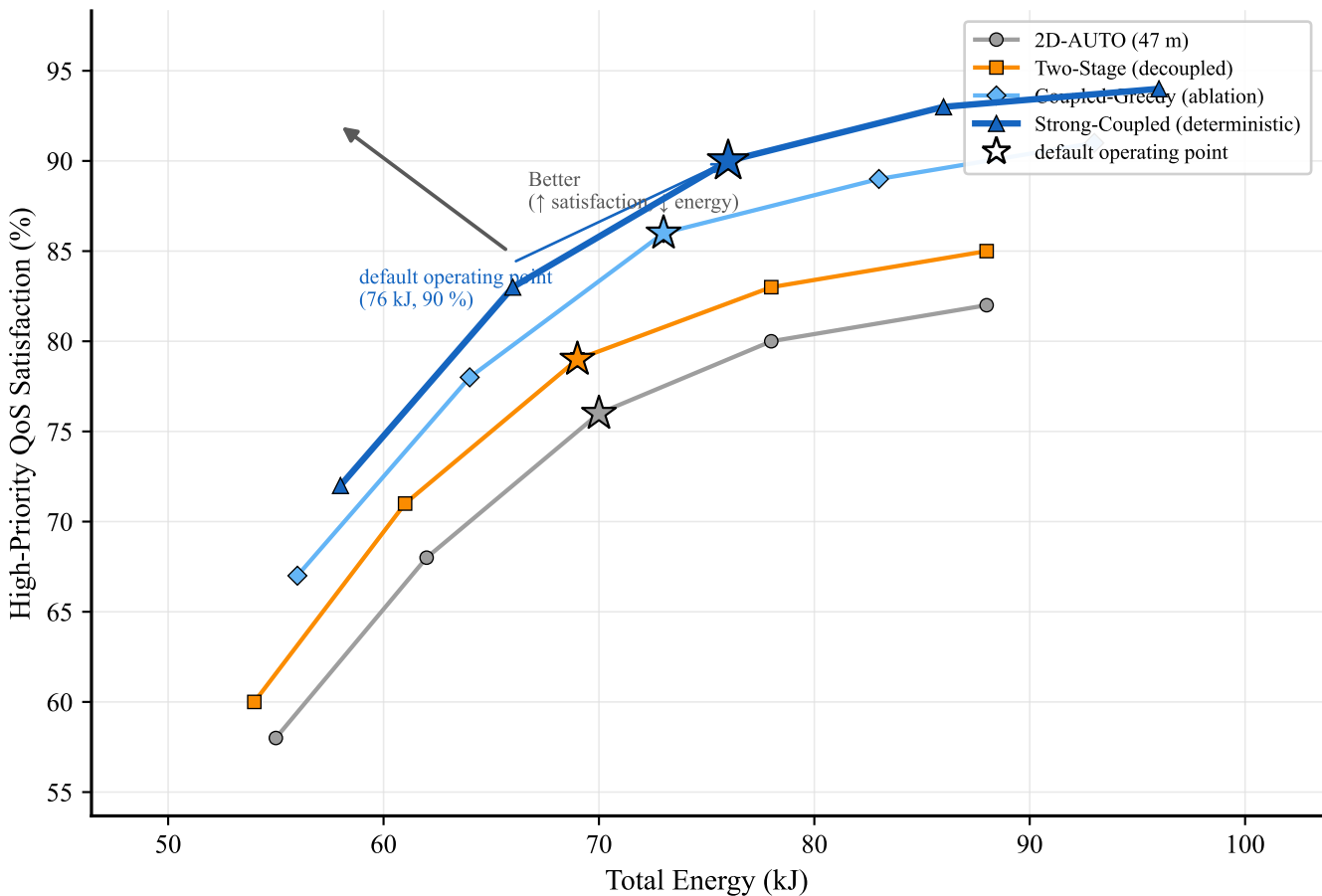
Energy vs. High-Priority Satisfaction Trade-off
