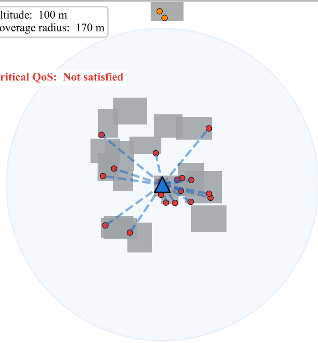
2D-AUTO
