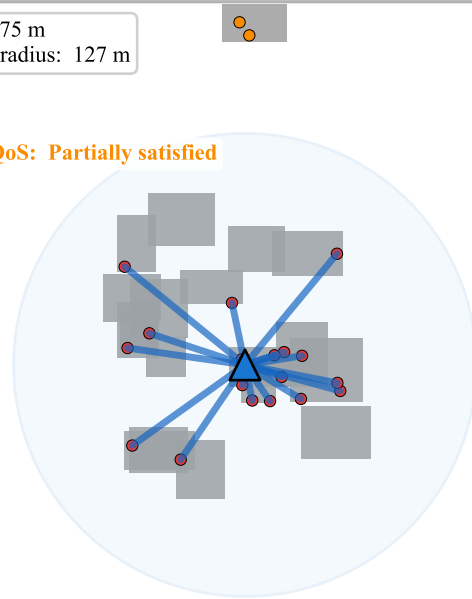
3D-GNN
