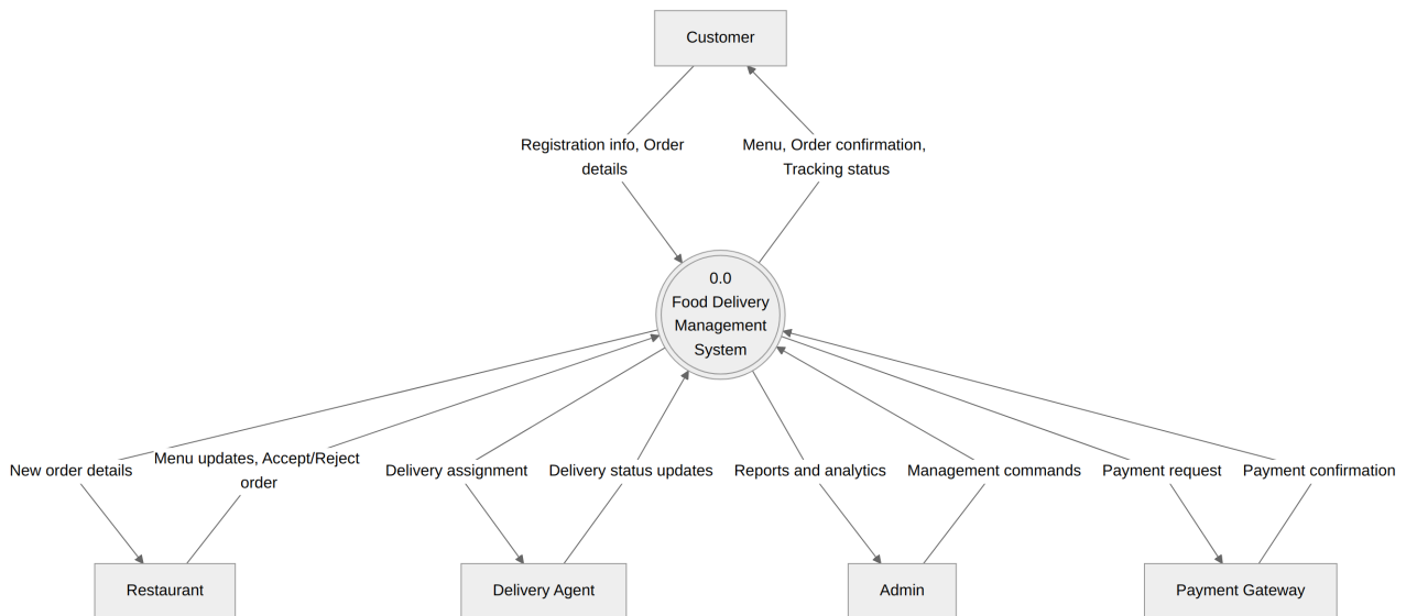
Figure 1: Context Diagram (Level 0)
