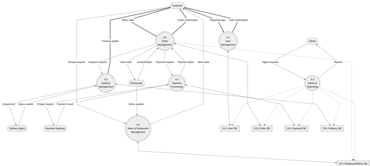
Figure 2: Level 1 DFD
