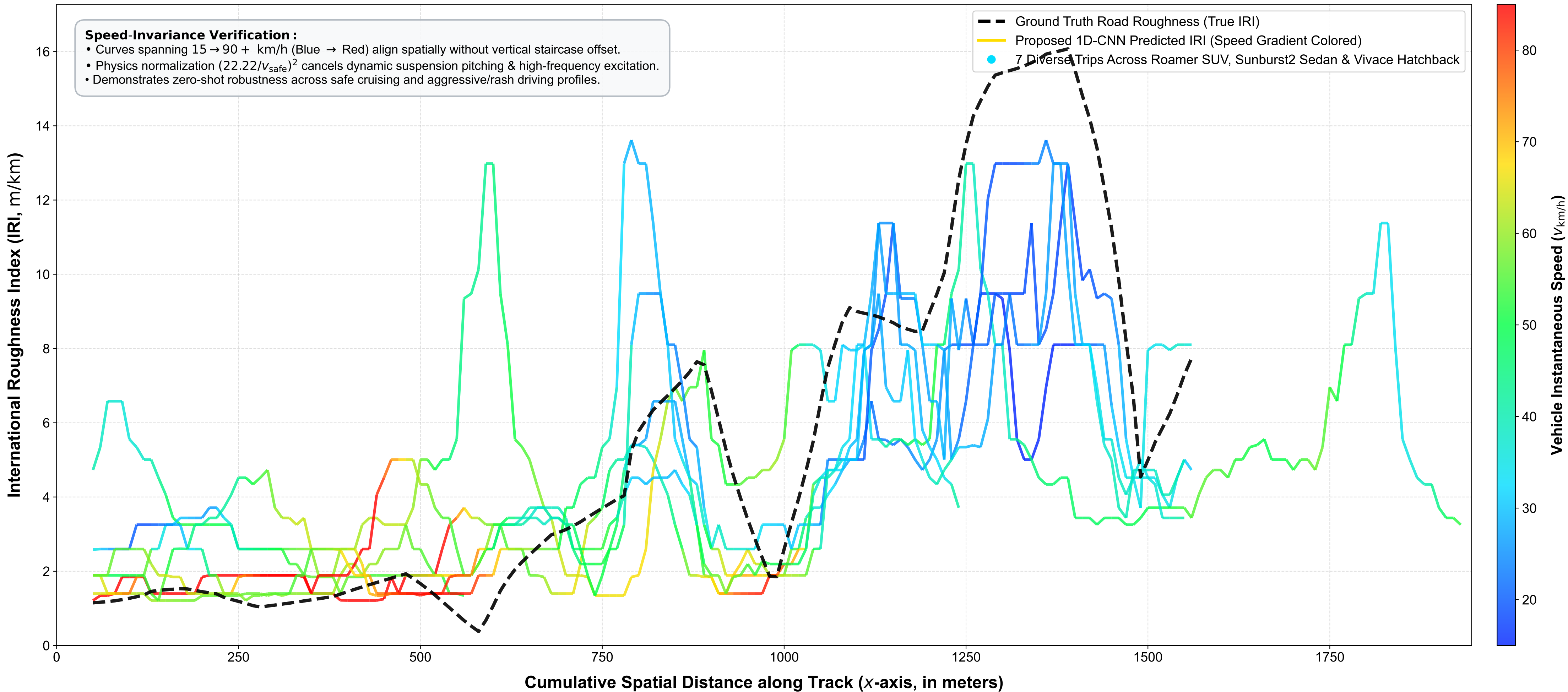
Multi-Vehicle Speed-Invariance Stress Test along Automation Test Track (Full 1.6 km Track)
