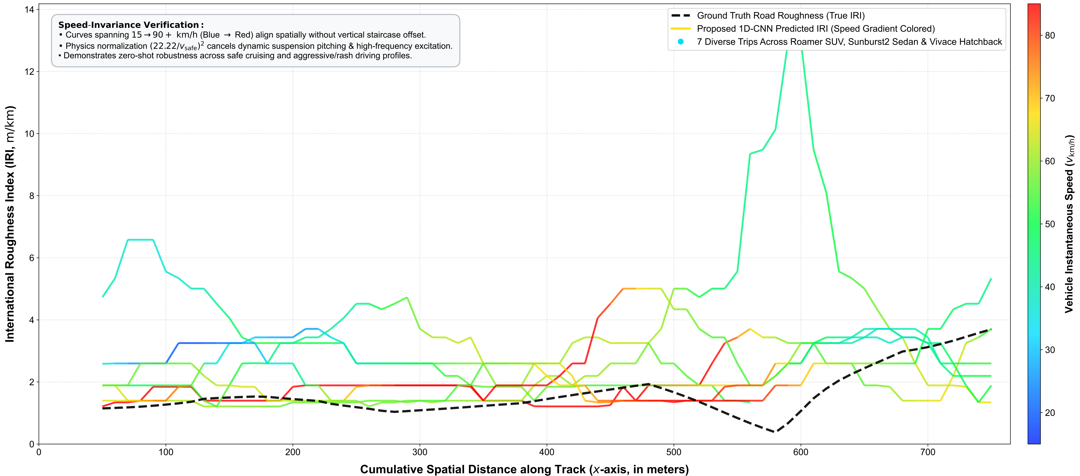
Multi-Vehicle Speed-Invariance Stress Test (0 → 750 m Reliable Alignment Stretch)
