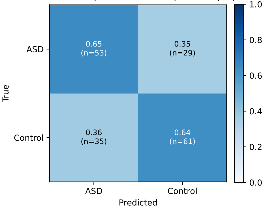
Confusion (row-normalized) — AAL (v1)
