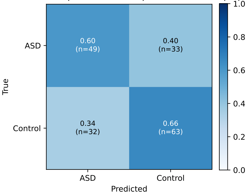
Confusion (row-normalized) — Schaefer100 (v1)
