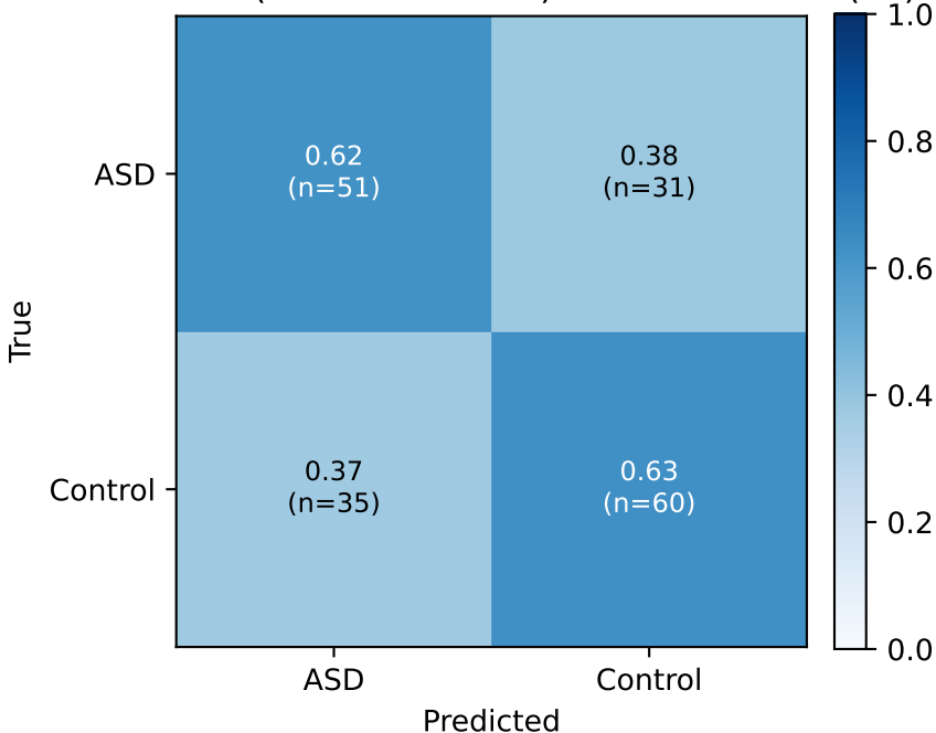
Confusion (row-normalized) — Schaefer100 (v2)
