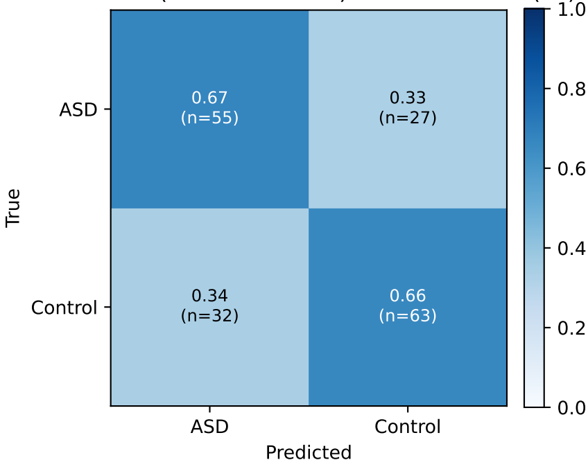
Confusion (row-normalized) — Schaefer200 (v1)
