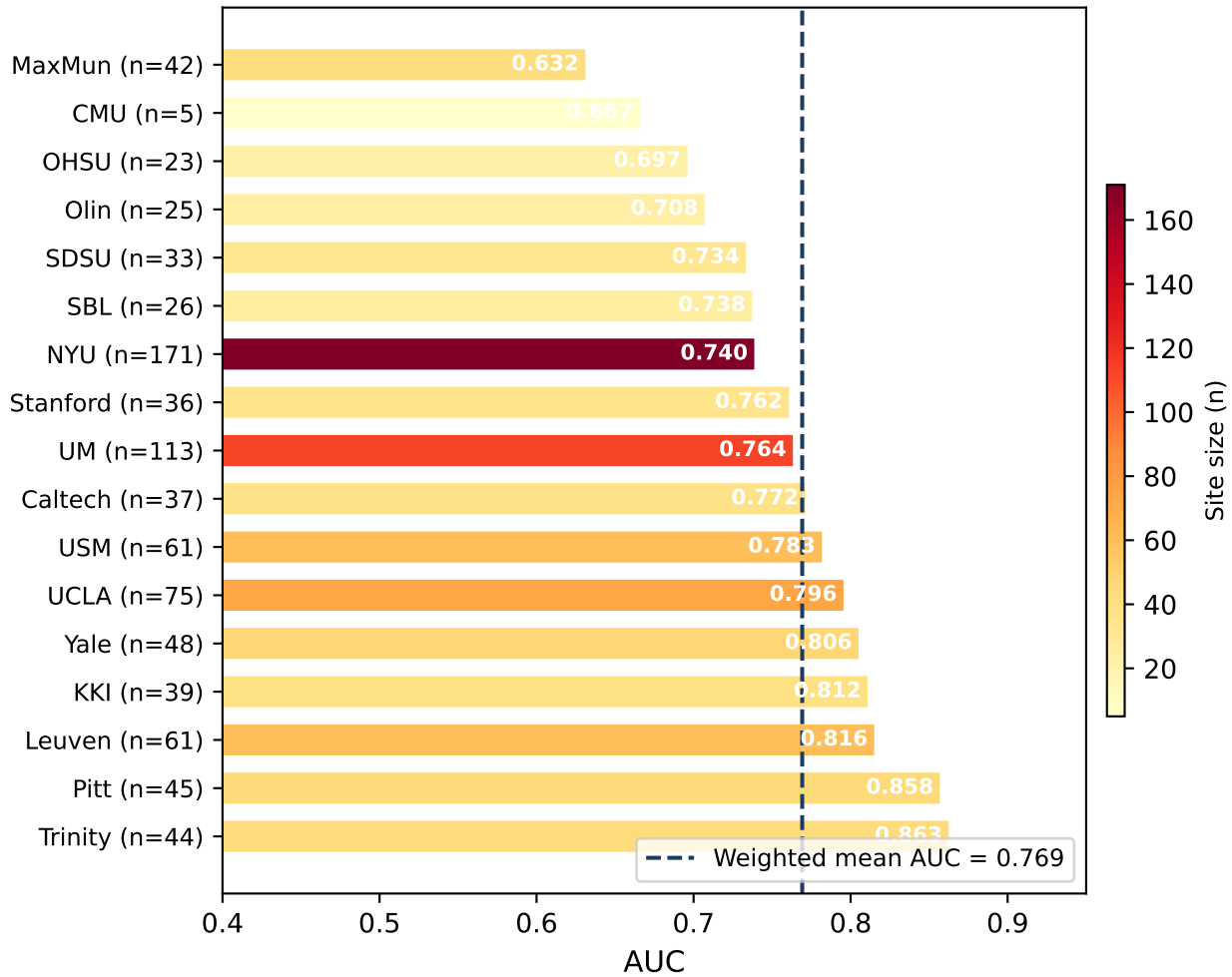
LOSO Per-Site AUC — Schaefer200 (v2)
