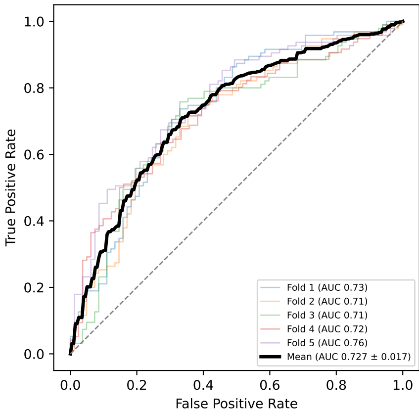
ROC — Schaefer200 (v1)
