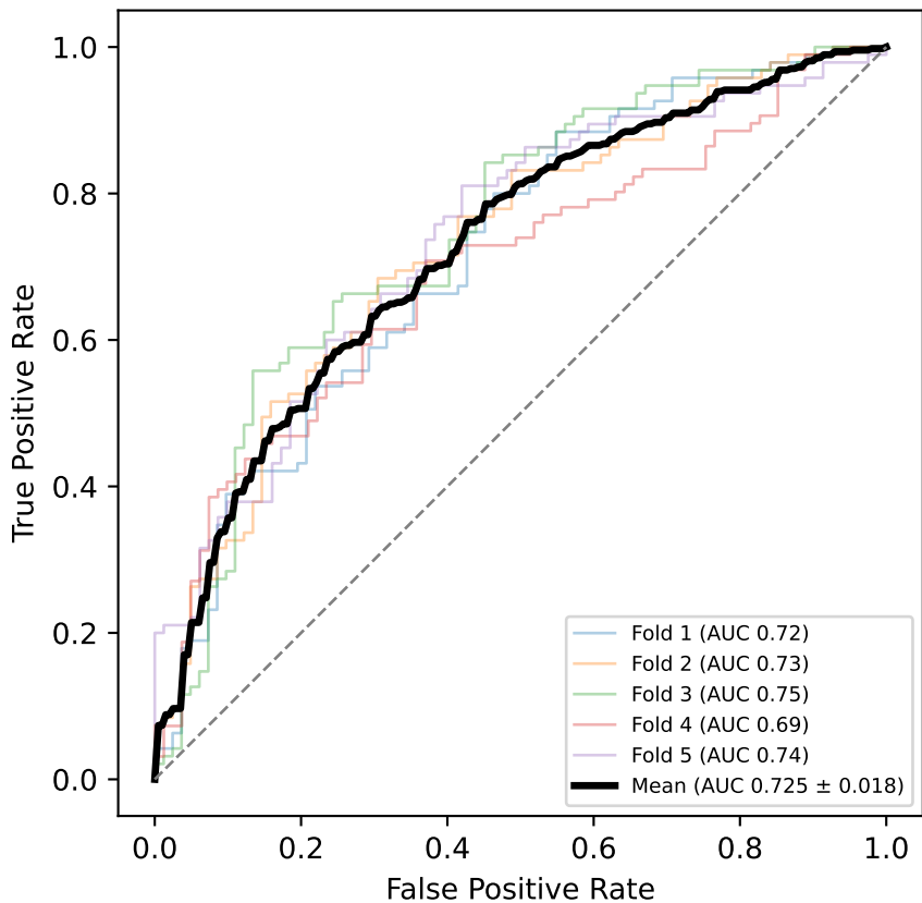
ROC — Schaefer400 (v1)
