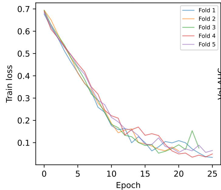
Training loss
