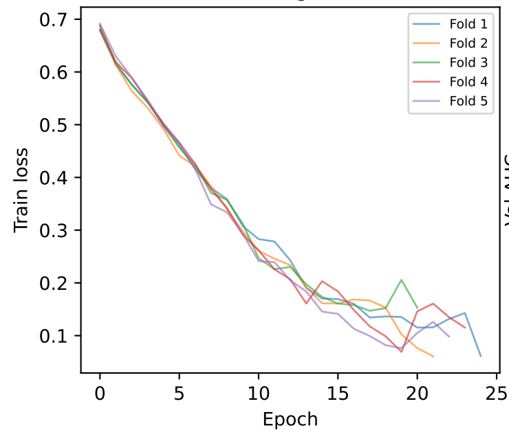
Training curves — Schaefer100 (v2)
