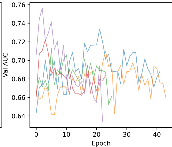
Training curves — Schaefer200 (v1) Training loss Validation AUC
