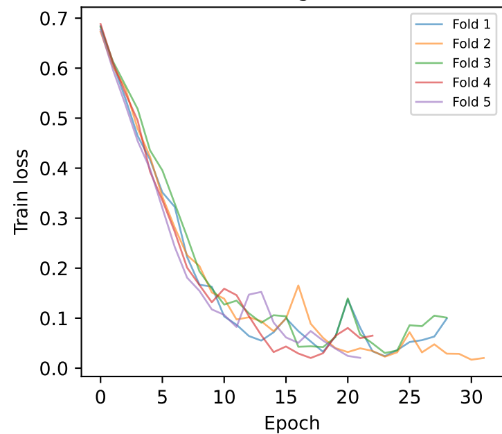
Training curves — Schaefer200 (v2) Training loss Validation AUC
