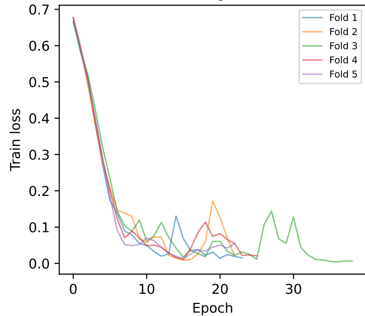
Training curves — Schaefer400 (v1) Training loss Validation AUC
