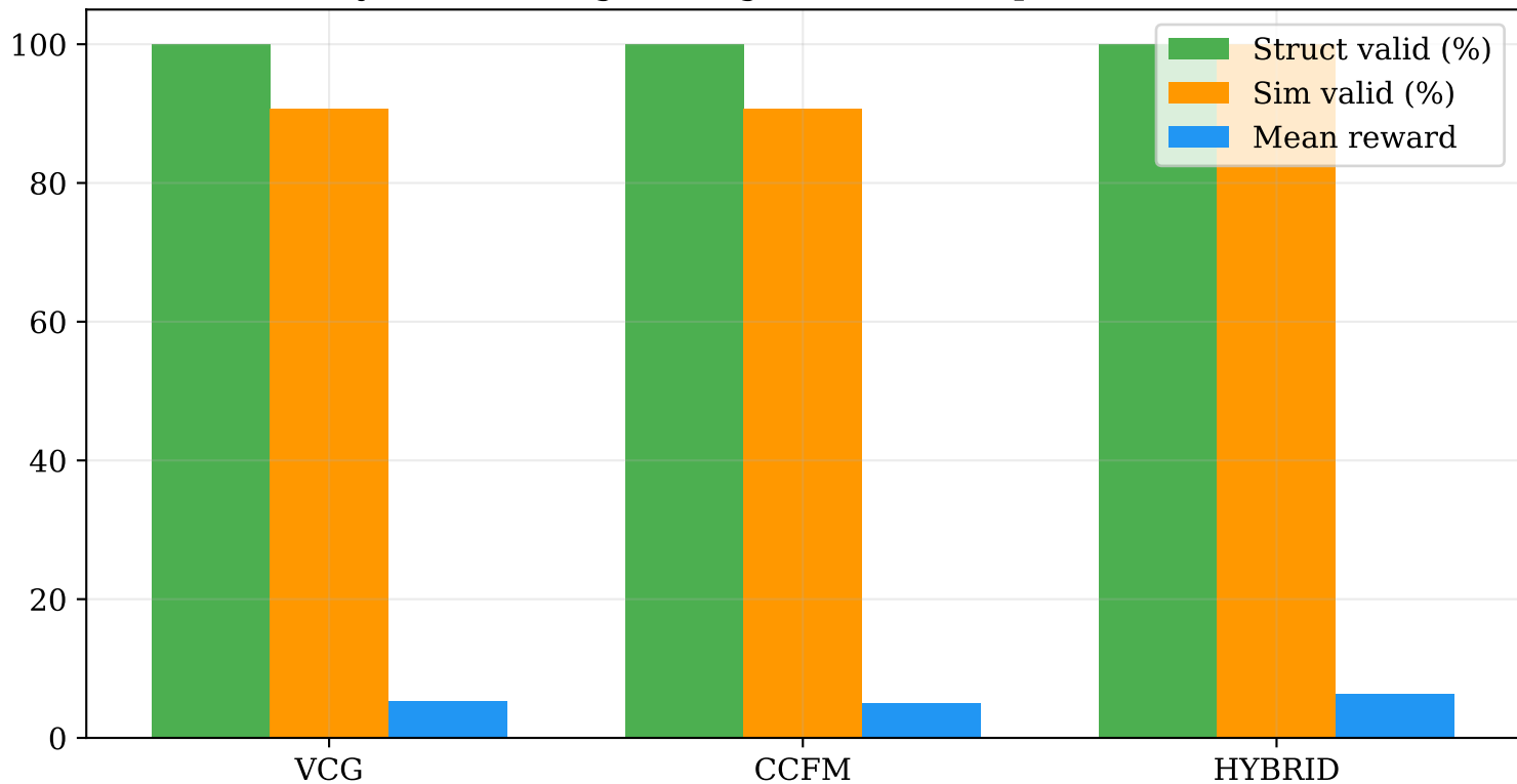
Hybrid Ranking vs Single-Source Graph Generators
