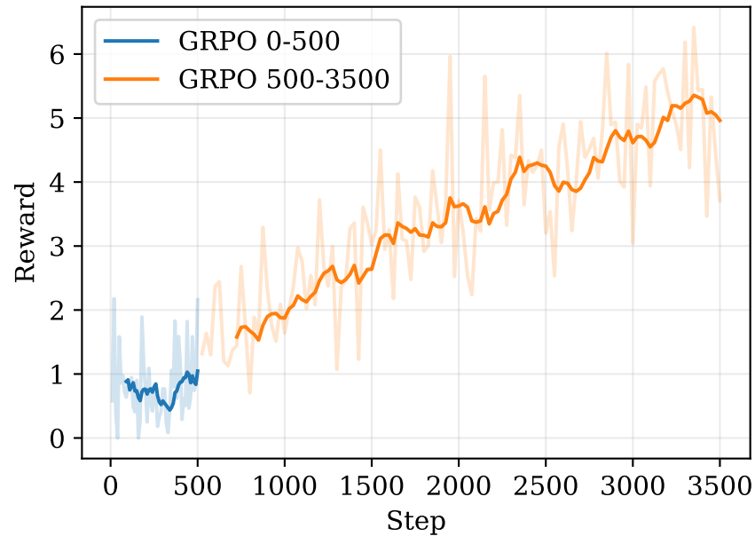
(a) Training Reward
