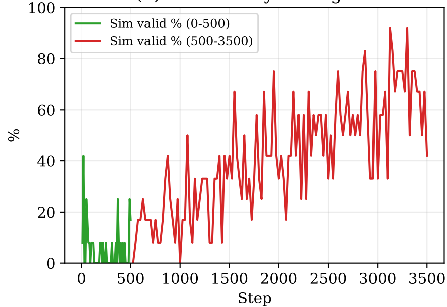
(b) Sim Validity During RL
