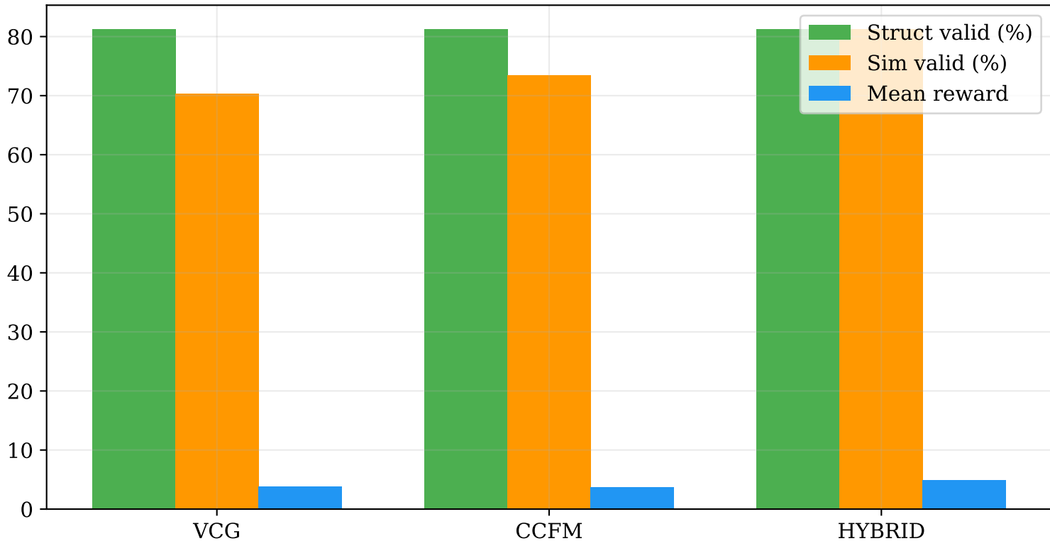
Hybrid Ranking vs Single-Source Graph Generators
