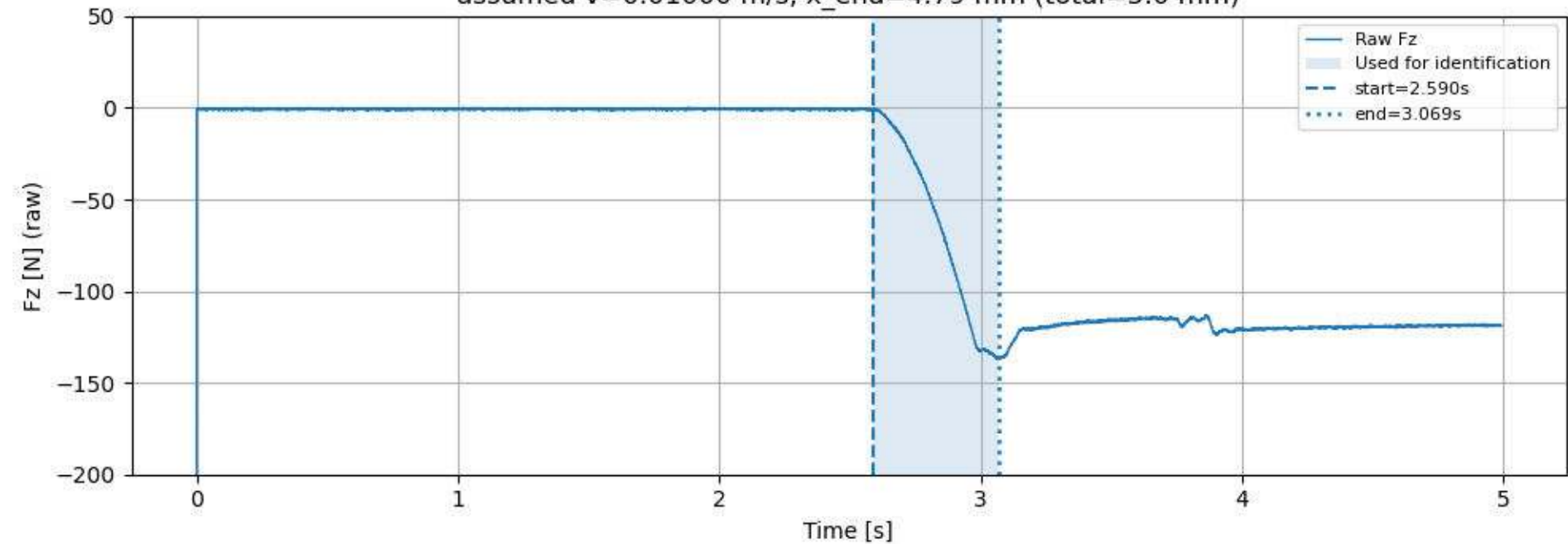
force_data_05.csv (High-resilience-Urethane) chosen range assumed v=0.01000 m/s, x_{\text{end}}=4.79 mm (total=5.0 mm)
