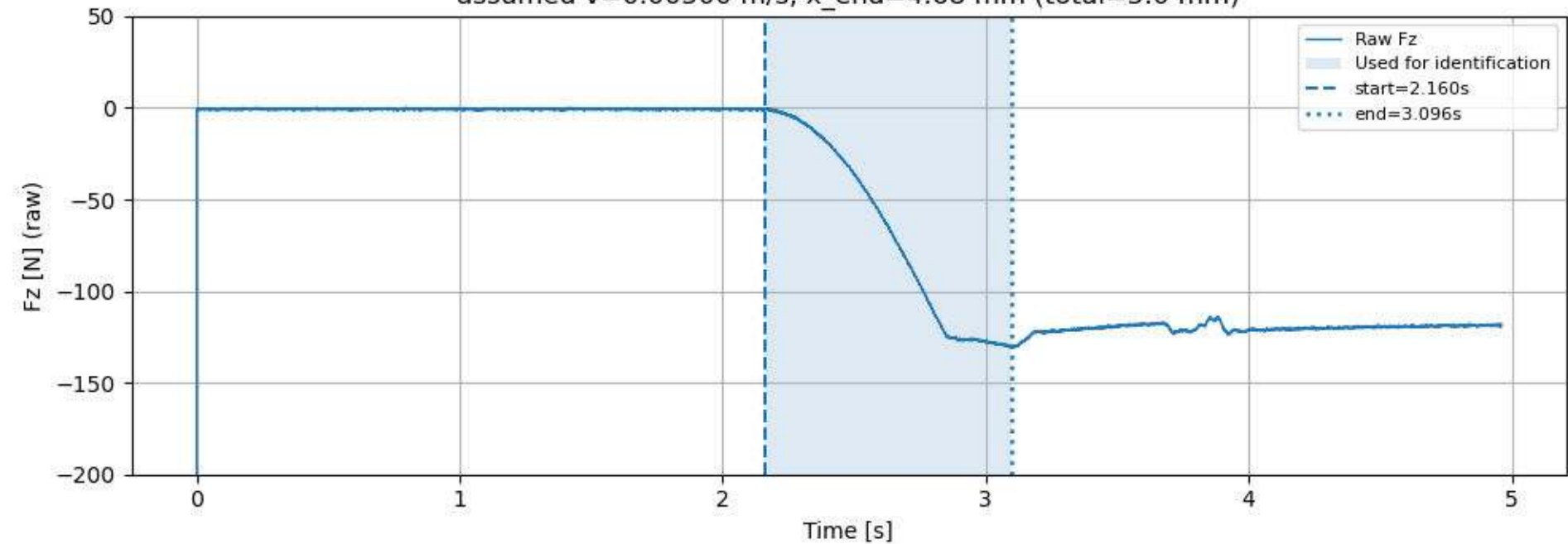
force_data_10.csv (High-resilience-Urethane) chosen range assumed v=0.00500 m/s, x_{\text{end}}=4.68 mm (total=5.0 mm)
