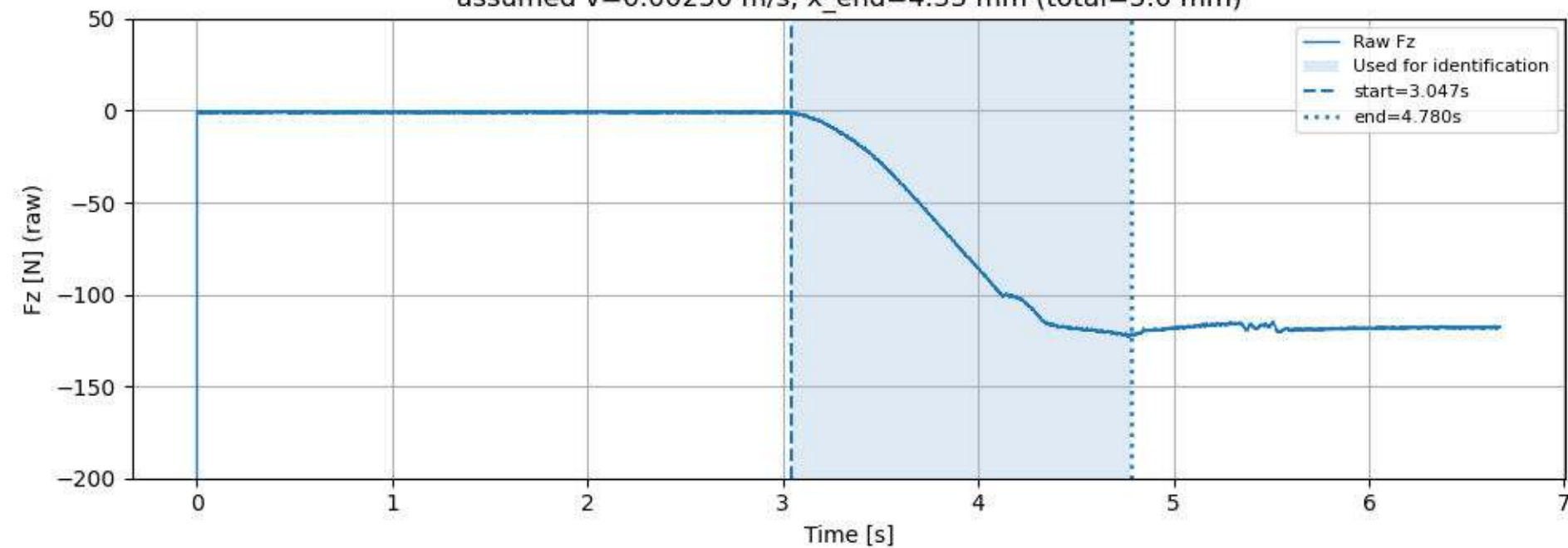
force_data_20.csv (High-resilience-Urethane) chosen range assumed v=0.00250 m/s, x_{\text{end}}=4.33 mm (total=5.0 mm)
