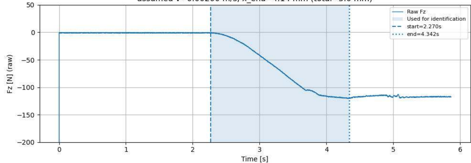
force_data_25.csv (High-resilience-Urethane) chosen range assumed v=0.00200 m/s, x_{\text{end}}=4.14 mm (total=5.0 mm)
