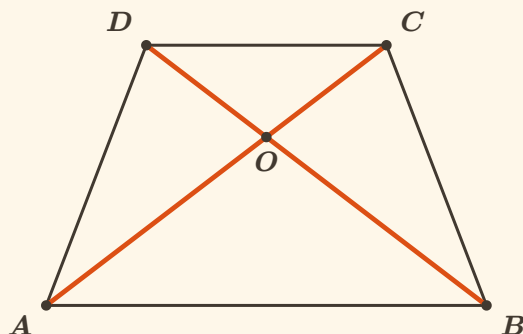
Trapezium ABCD with AB parallel to DC
