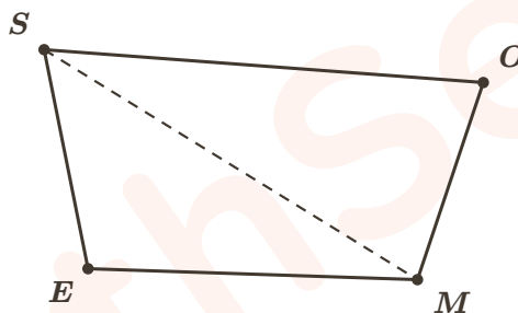
Diagonal SM divides the quadrilateral into two triangles
