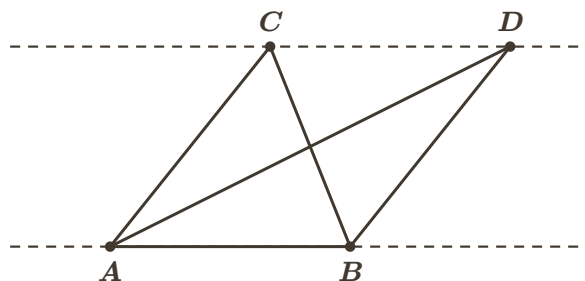
Triangles ABC and ABD are on the same base AB and between the same parallels
