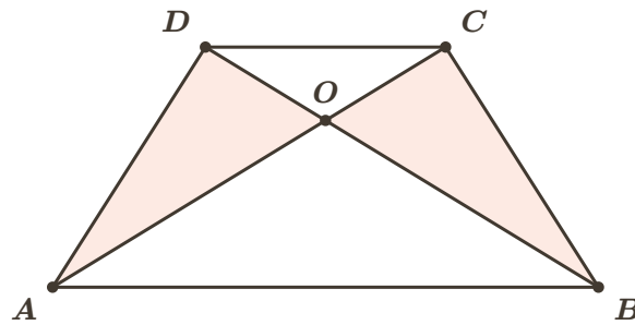
Trapezium ABCD: the shaded triangles AOD and BOC have equal areas
