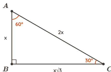
A 30-60-90 triangle with sides x , x\sqrt{3} and 2x
