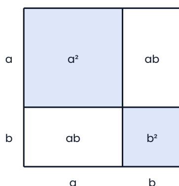
A square of side a + b
