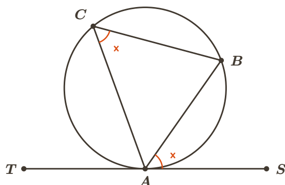
Angle BAS between the tangent and the chord equals angle ACB in the alternate segment
