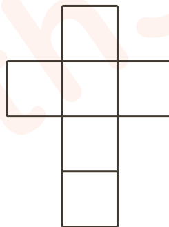
A net of a cube
