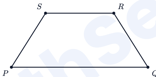
Isosceles trapezium: PQ is parallel to SR and PS = QR
