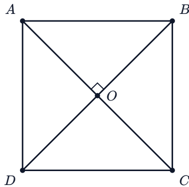
Square: equal diagonals meeting at 90^\circ
