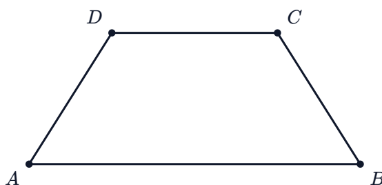
Isosceles trapezium: AB is parallel to DC and AD = BC
