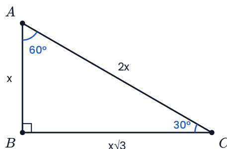
A 30-60-90 triangle with sides x , x\sqrt{3} and 2x
