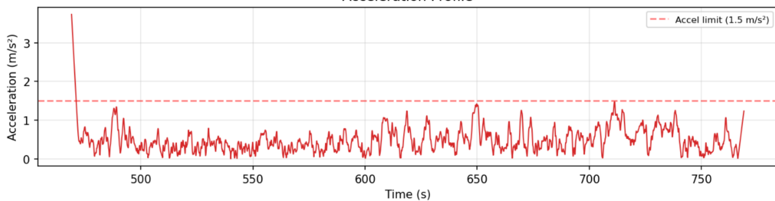
Acceleration Profile
