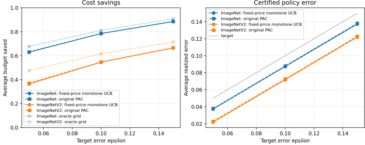
Figure 1: Offline sweep over target error levels. After exploiting the single-source monotonicity, the fixed-price rule is nearly indistinguishable from the original scalar PAC baseline; the remaining gap comes from using a fixed threshold grid rather than the exact calibration-order threshold.
