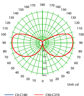
Luminous Intensity Distribution Curve - 4004.204.1F4
