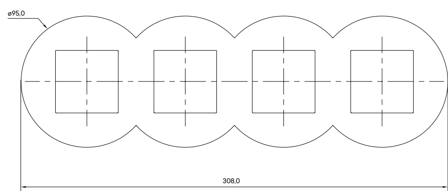
Ref. 43940 T - SV Quádruplo
