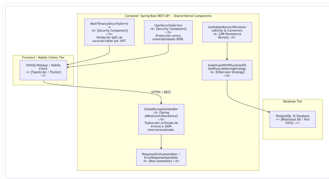
Figura 5: Component Diagram (C4 Level 3) – Shared Kernel
