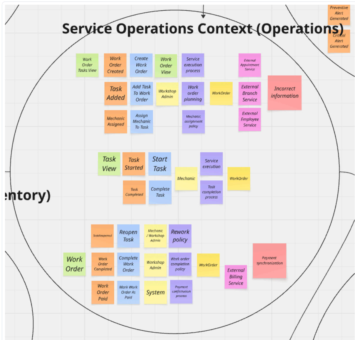
Figura 9: Candidate Bounded Context — Service Operations
