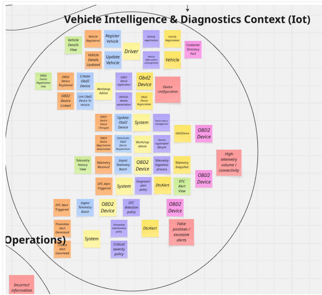
Figura 14: Candidate Bounded Context – Vehicle Intelligence & Diagnostics.
