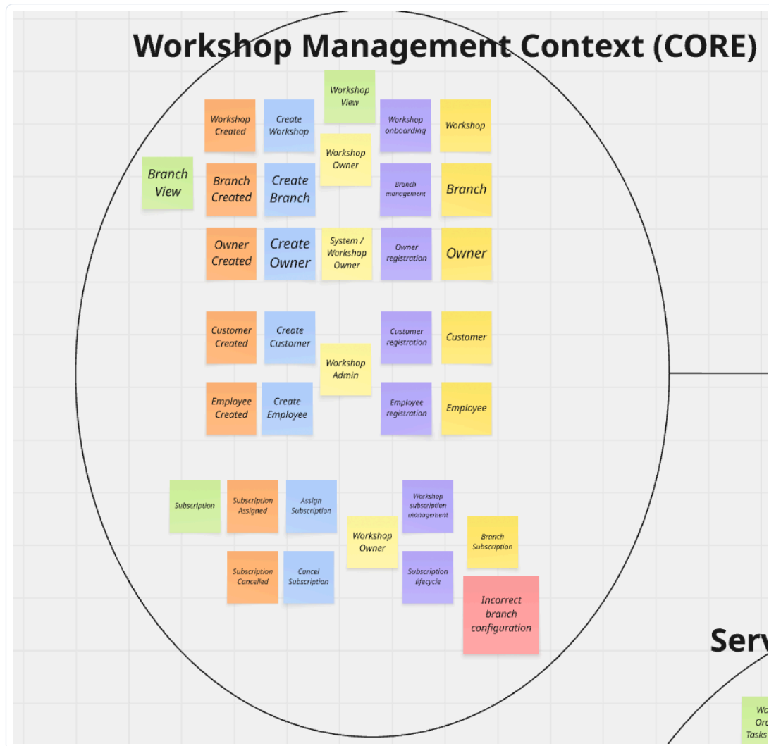
Figura 12: Candidate Bounded Context – Workshop Management.
