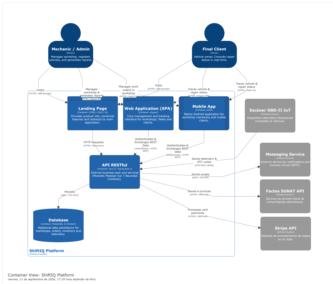
Figura 34: Diagrama de Contenedores – ShiftIQ Platform.
