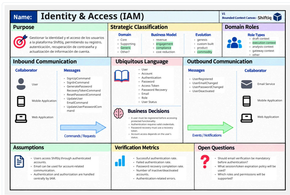
Figura 24: Bounded Context Canvas – Identity & Access.
